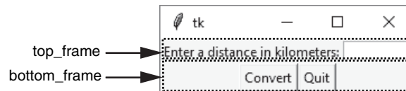
Figure 13-14 The window organized with frames
